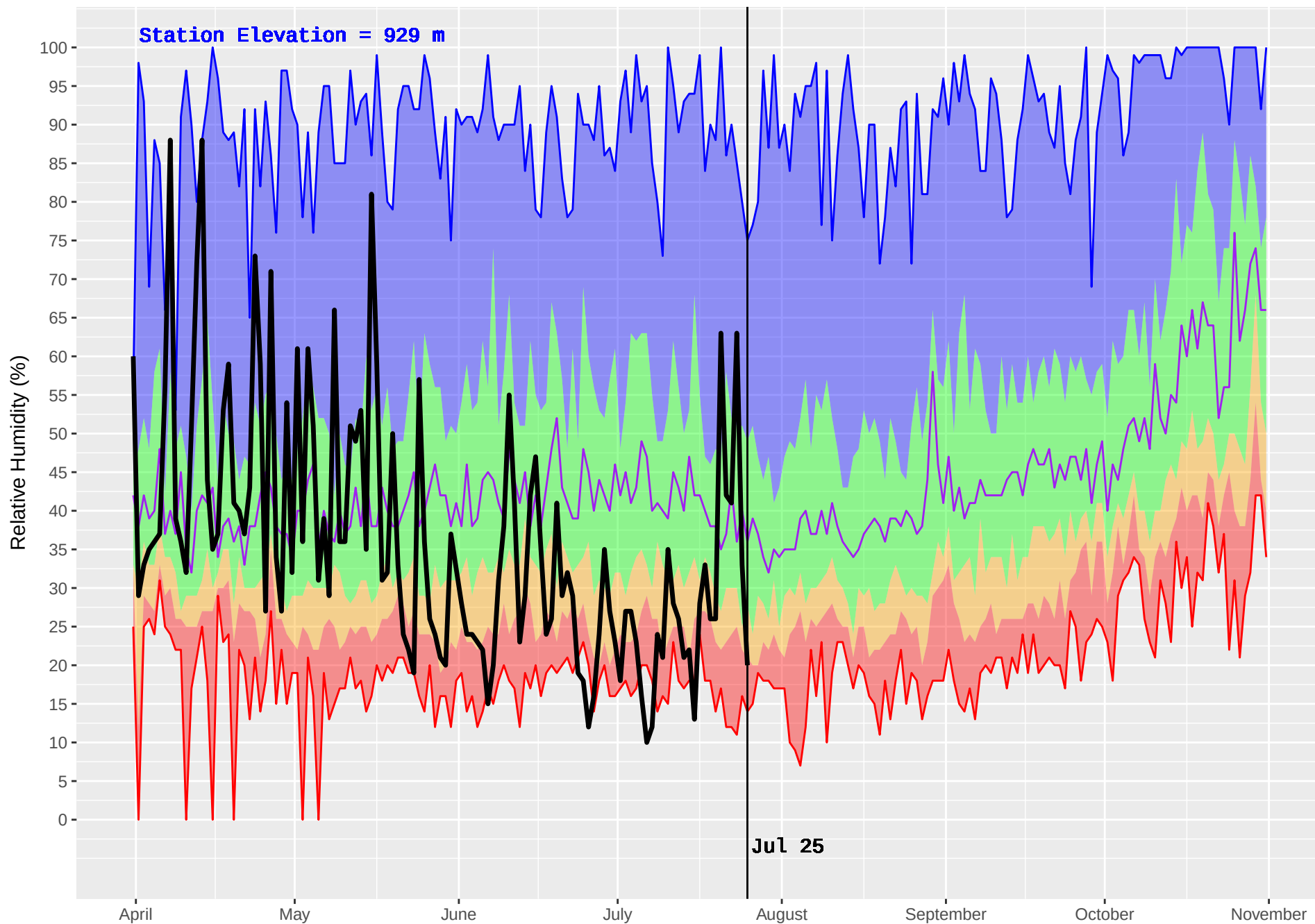
RISKE CREEK (210) : Historical (1980–2016) and Current (2017) Noon Relative Humidity
