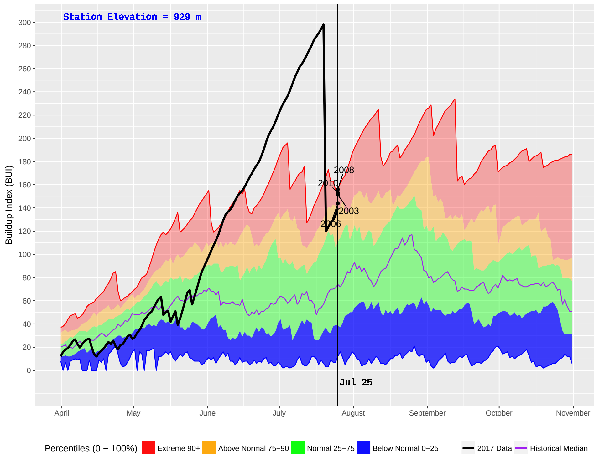
RISKE CREEK (210) : Historical (1980–2016) and Current (2017) Noon Buildup Index (BUI)
