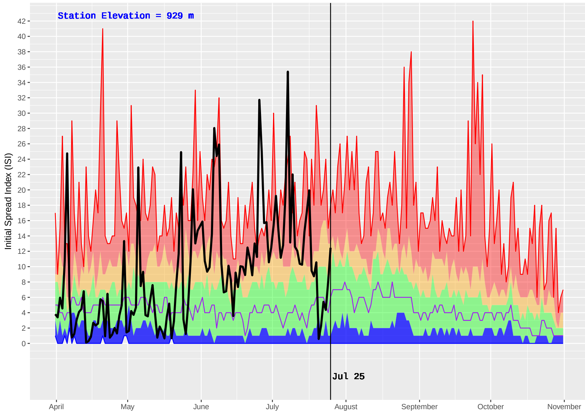
RISKE CREEK (210) : Historical (1980–2016) and Current (2017) Noon Initial Spread Index (ISI)
