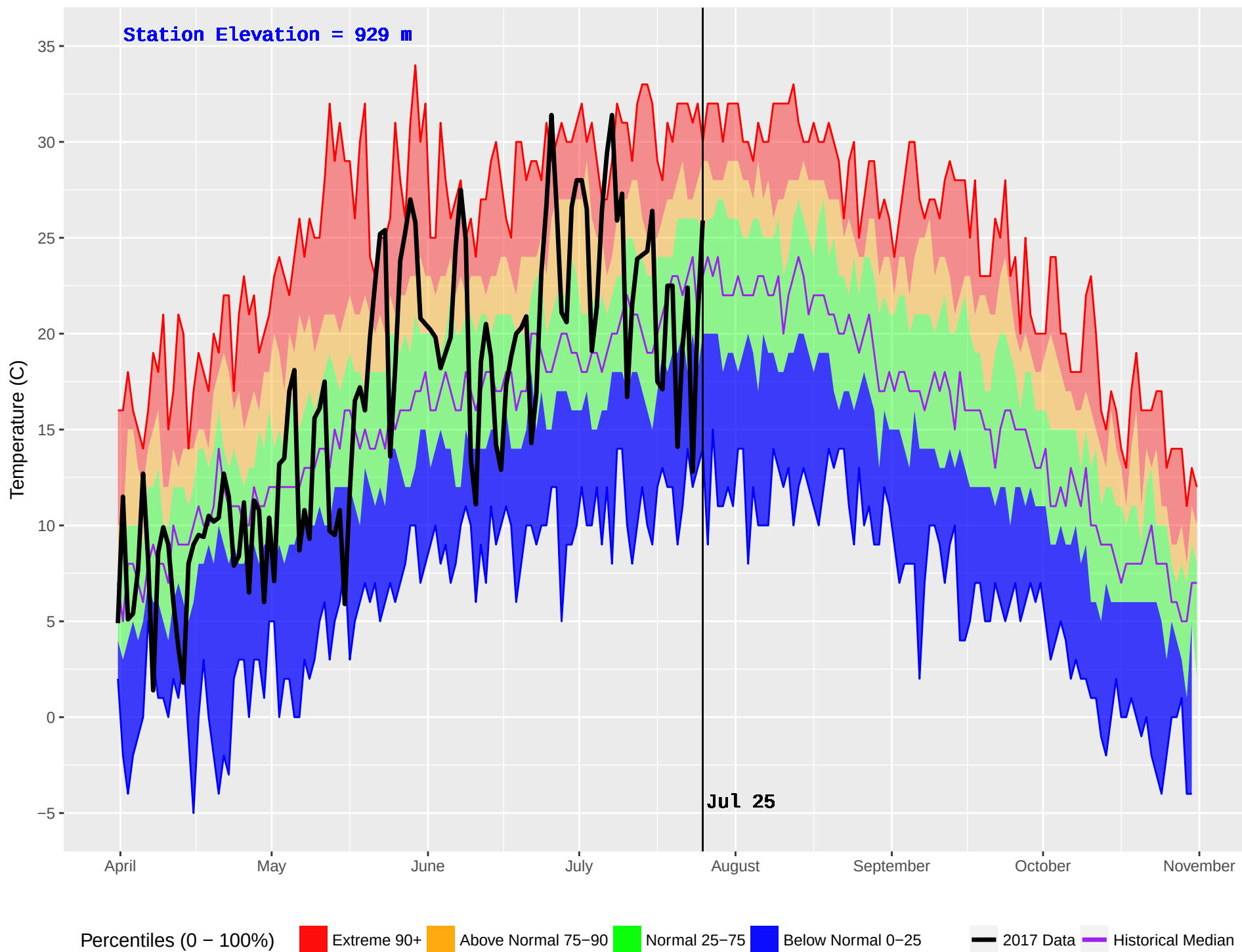
RISKE CREEK (210) : Historical (1980–2016) and Current (2017) Noon Temperature
