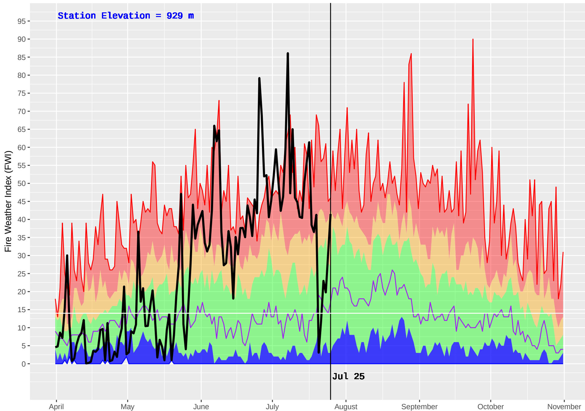
RISKE CREEK (210) : Historical (1980–2016) and Current (2017) Noon Fire Weather Index (FWI)
